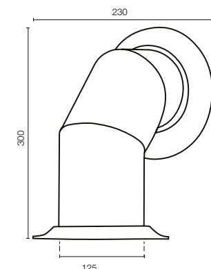
Pipe to suit Horizon Stove
