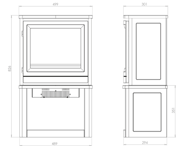
Horizon Stove with Log Store
