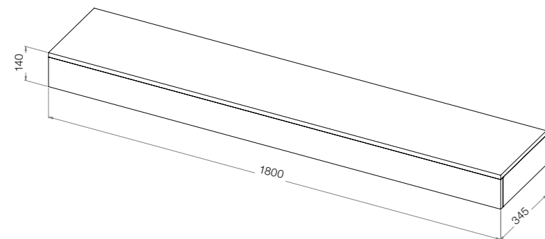
Canova Plinth to suit VS150 / VS150+
