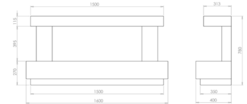
Zenith Suite to suit VS100 / VS100+
