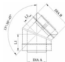
Pictured above is the 30° elbow
